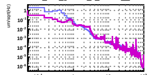
SBE_EIB_ground_z_200Hz__FFT
