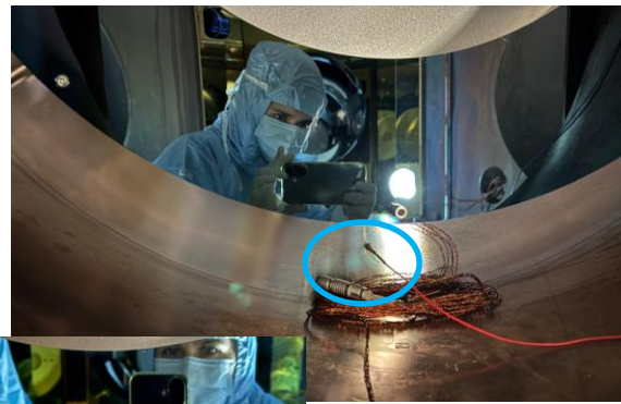
R3: horizontal position on the vacuum vessel
