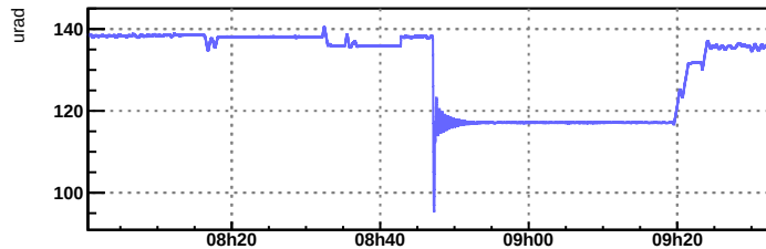
Sc_IB_BENCH_TY_mean__TIME
