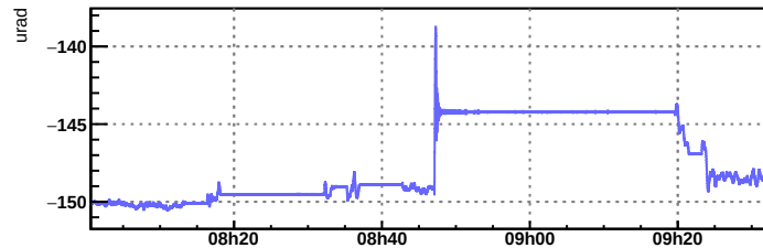
Sc_IB_MAR_TZ_mean__TIME
