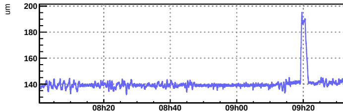
Sa_PR_F0_X_mean__TIME
