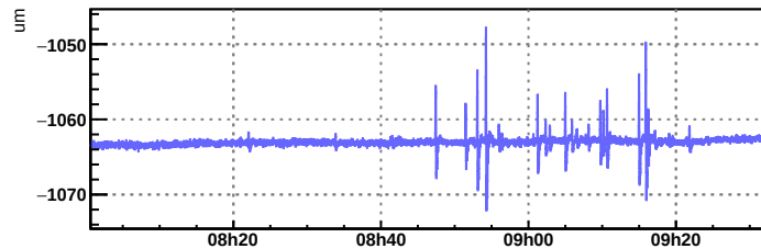
Sc_PR_F7_Y_mean__TIME
