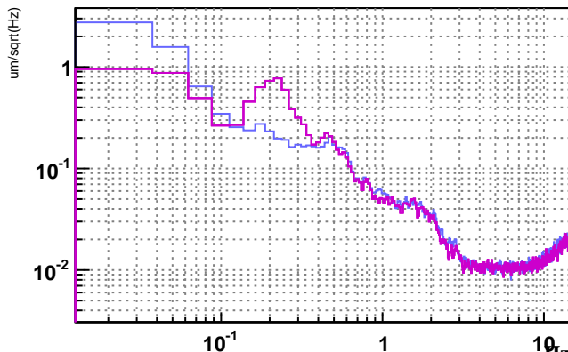
V1:SDB2_LC_Z_err_ground_corrected__FFT
