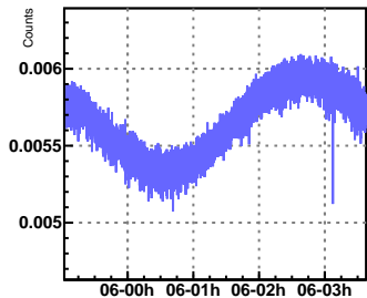
V1:EPRB_B4_PC_112MHz_PDH_PWR__TIME
